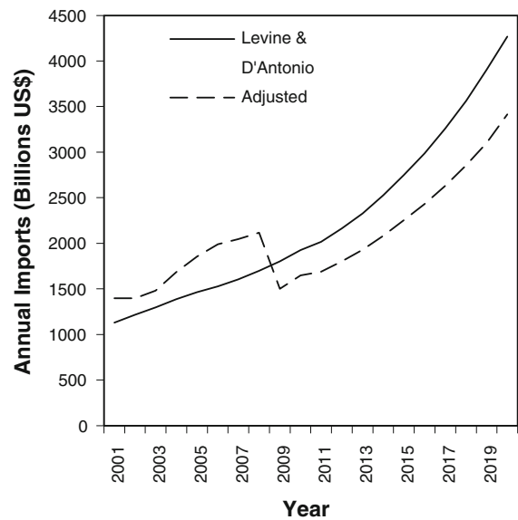
Fig. 1 Annual import curve based on data used by Levine and D'Antonio (2003) and the adjusted import curve utilized in this study. The annual import values are in 2008 US dollars
