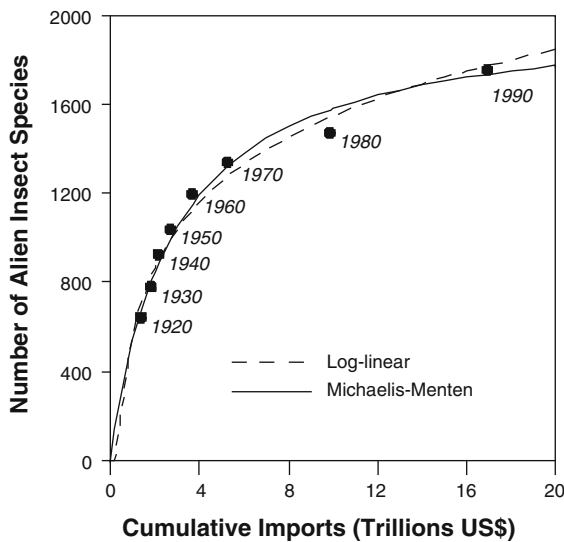
Fig. 3 Re-parameterized log-linear and Michaelis–Menten models relating cumulative US imports to the establishment of alien insect species. The cumulative import values are in 2008 US dollars
