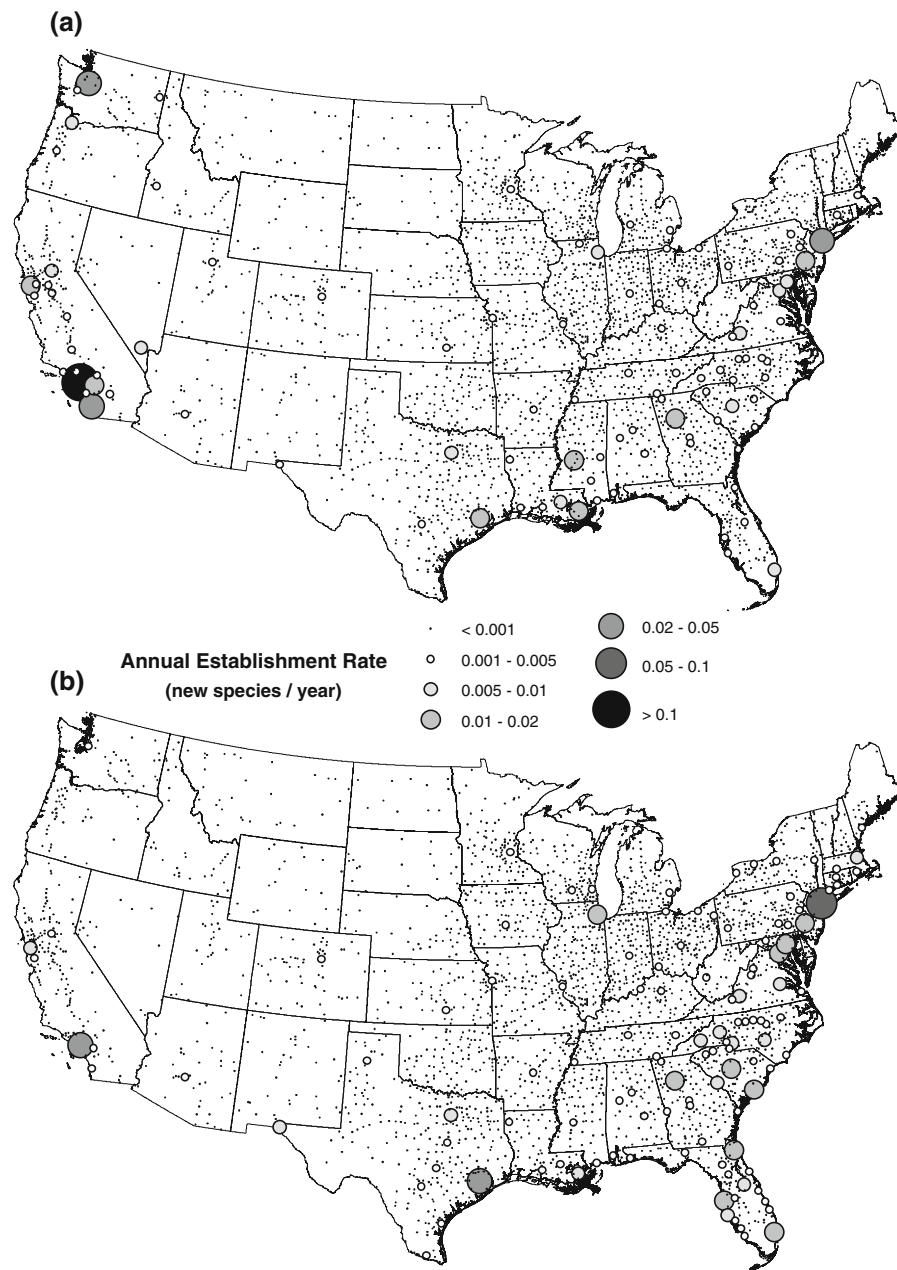
Fig. 5 Annual forest insect establishment rates in US urban areas, based on imports of relevant commodities from a specific origin region: a Asia (i.e., FAF region “Asia E&S”); b Europe. Rates were estimated using 2010 FAF projections
