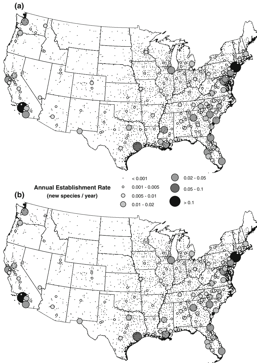
Fig. 4 Annual alien forest insect species establishment rates in US urban areas, based on imports of relevant commodities from all world regions of origin: a rates estimated using 2010 FAF projections and the 2001–2010 mean annual rate of alien
