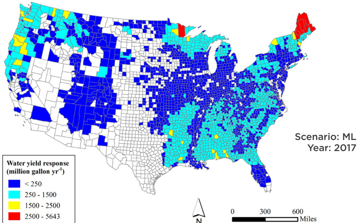
Figure 7.7 | WaSSI modeled projected response of mean annual water yield to reference under the ML 2017 harvesting scenario across the United States showing A, absolute response in million gallons per year and B, relative response by percentage
