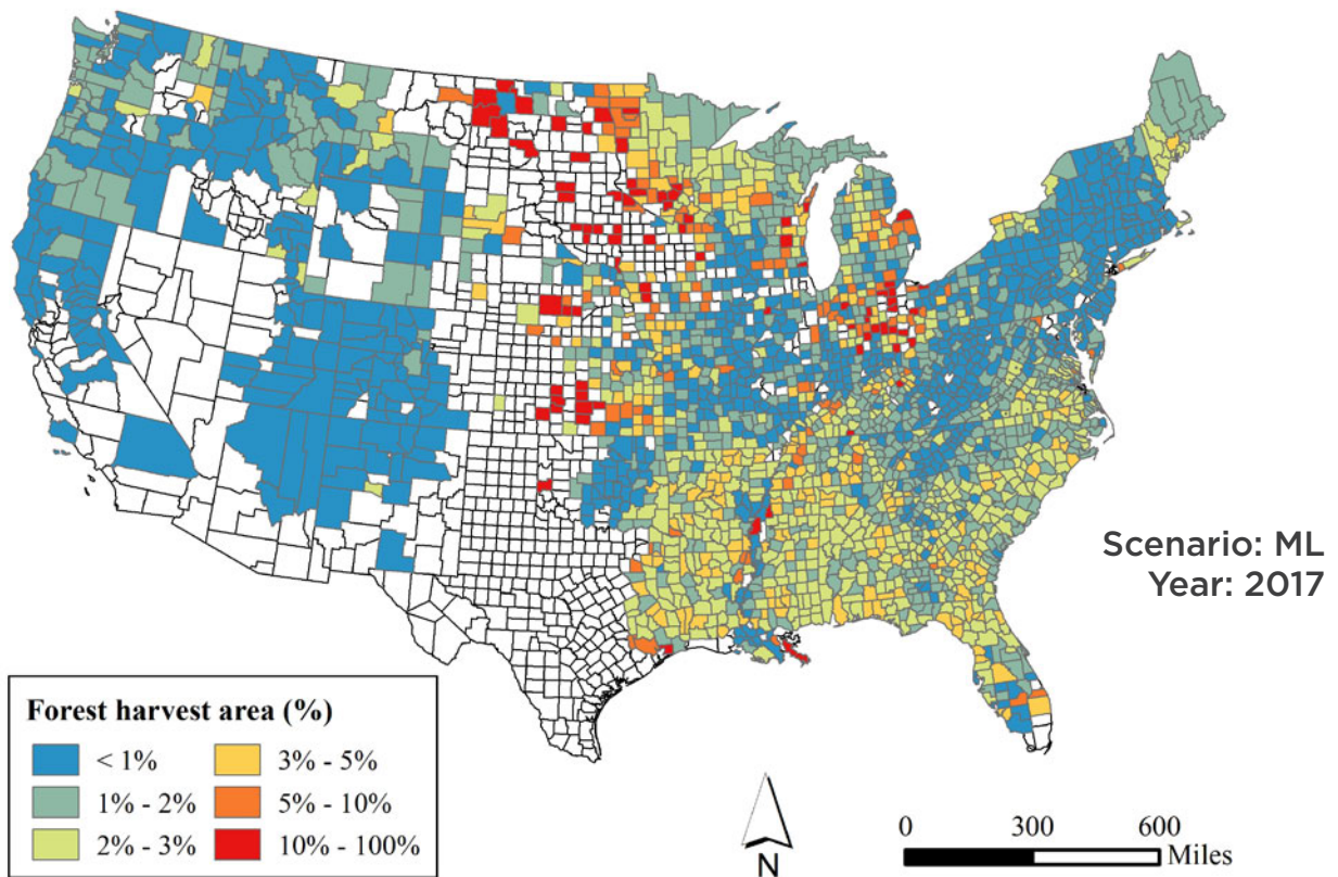
Figure 7.2 | Forest harvesting percentage (clearcutting plus thinning) under three biomass scenarios in 2017 and 2040
