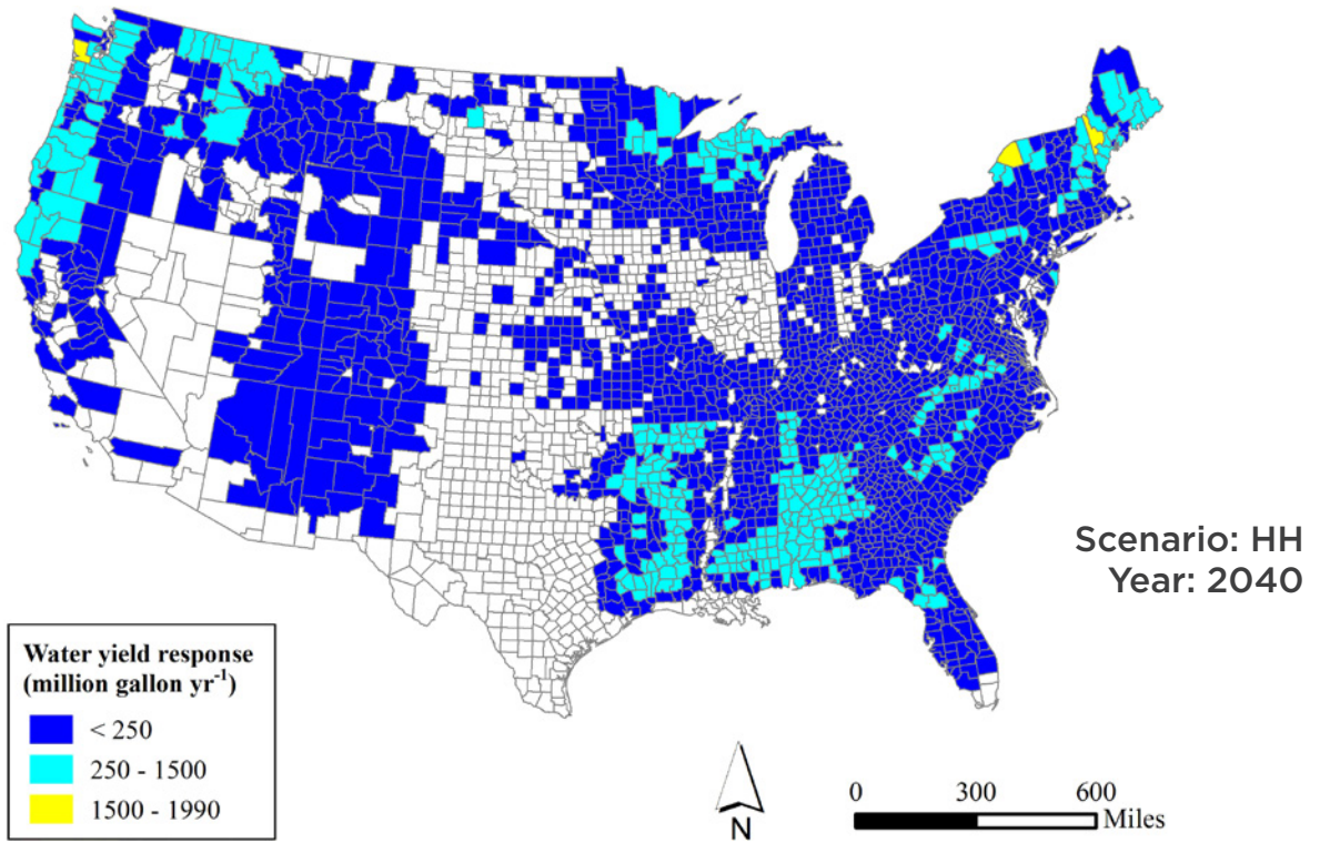
Figure 7.9 | WaSSI modeled projected response of county-level mean annual water yield under the HH 2040 harvesting scenario across the United States, showing A, absolute response in million gallons per year and B, relative response as a percentage change from reference conditions
