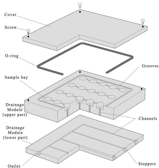
Figure 1. The schematic drawing of Delrin holder for acetone pretreatment.
