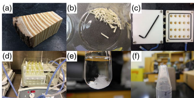
Figure 2. The main steps of \alpha -cellulose extraction: (a) a surfaced wood wedge for sampling; (b) wood slivers for \alpha -cellulose extraction; (c) slivers in Delrin holders with/without the lid (pretreatment); (d) \alpha -cellulose extraction by MSISS; (e) extracted \alpha -cellulose in chips and fibers; (f) homogenized and dried \alpha -cellulose. (All photos by W. Lin. The glass tube in (e) and plastic vial in (f) are for demonstration only and were not used in the experiment.)
