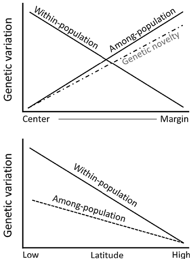
Fig. 2 Diagram showing hypothesized differences in within-population ( \alpha -diversity) and among-population genetic variation ( \beta -diversity) along the central–marginal and latitudinal gradients across species ranges. Within- and among-population genetic variations show contrasting patterns from the centre to margin due to joint effects of population density (and size) and isolation (Lammi et al. 1999; Zakharov & Hellmann 2008; top). Also, because range margins may be more dynamic in terms of expansion or contraction and have greater chances of hybridization, the adaptive genetic novelty would be higher at range margins, especially the advancing (or colonizing) margins. Everything else being equal (i.e. population size, density, isolation), within- and among-population (given the same levels of isolation and distances among them) genetic diversity may show similar patterns along latitude (Martin & McKay 2004), yet their relative positions and strength would be highly species-specific and may depend on how each is measured (Schrey et al. 2011; bottom). The latitudinal trends are based on the assumptions that (i) the same mechanisms responsible for the latitudinal patterns in overall species diversity also lead to similar patterns in within-species diversity (Mittelbach et al. 2007; Miller et al. 2010), and (ii) much genetic variation and resources are left at lower latitudes following poleward species migration (e.g. after glaciations).
