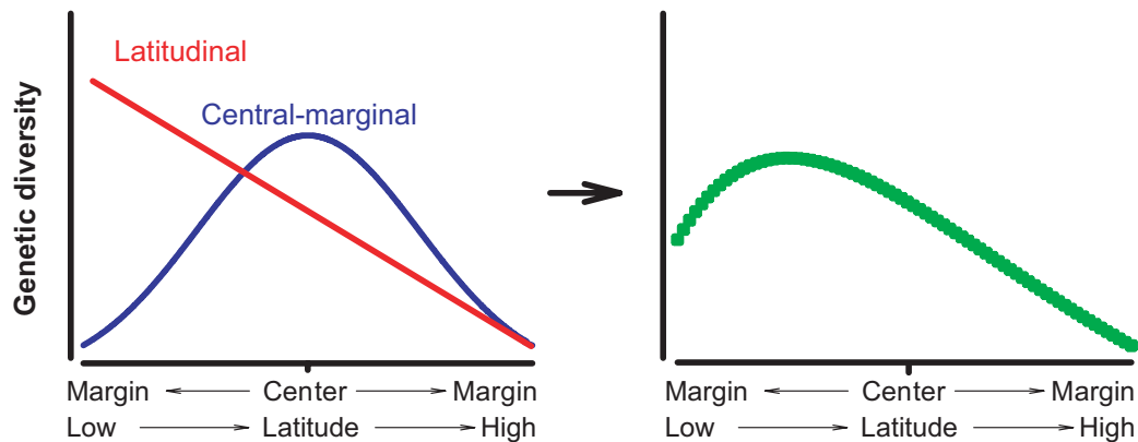
Fig. 1 An example of species with a general central–marginal (C–M) decline in density showing how within-population genetic diversity might vary across the whole species range (i.e. from centre to margin) and with the latitude (i.e. low to high). If the latitudinal pattern in genetic diversity is detectable (especially for species with large ranges or latitudinal extents), the C–M pattern trend (similar to or may be related to the geometric constraint or mid-domain effect; Colwell et al. 2004; Miller et al. 2010) is enhanced or overwhelmed by the latitudinal pattern in the higher latitudinal portion of the species range but weakened or obscured in the lower latitudinal portion. The interactive effects of latitudinal and C–M processes (left) lead to the intermediary pattern often observed in the field with genetic diversity peaks at lower portion of the species' latitudinal extents (right).
