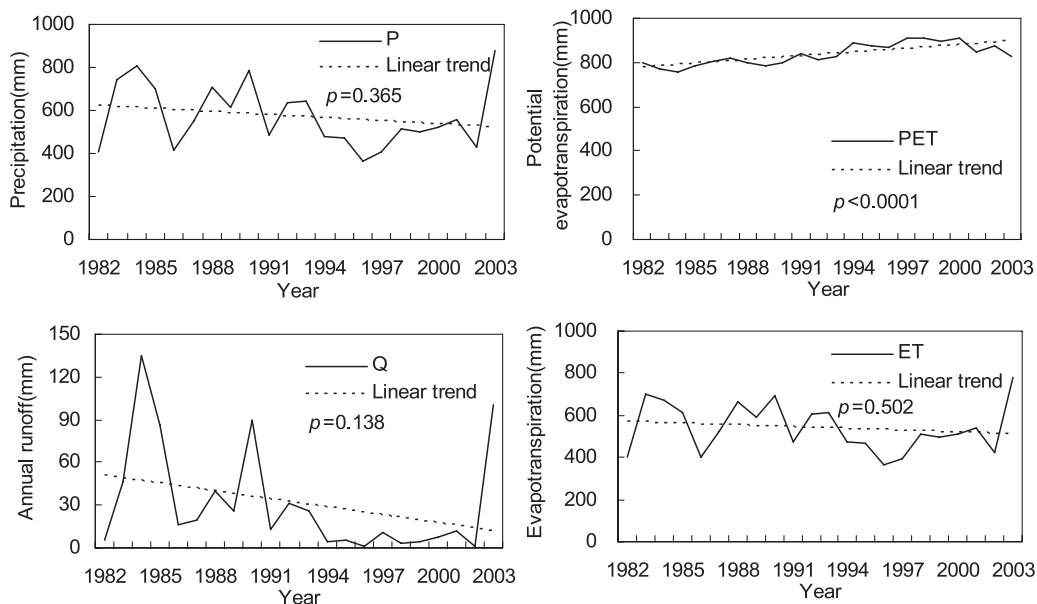
FIGURE 4. Annual Variation of P , PET, ET, and Q With Their Respective Linear Regression Line.
