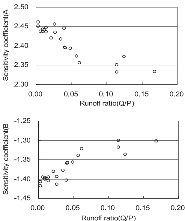
FIGURE 7. Scatter Plot of Sensitivity Coefficient Against Runoff Ratio.
