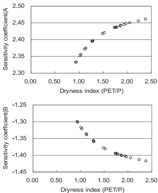
FIGURE 6. Scatter Plot of Sensitivity Coefficient Against Dryness Index.
