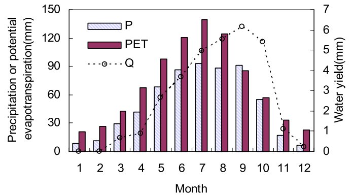
FIGURE 3. Monthly Distribution of Averaged P , Q , and PET.
