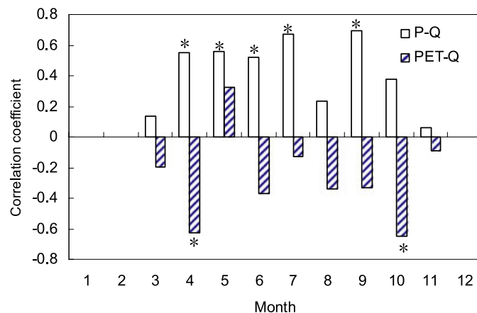
FIGURE 5. Correlation Coefficient for Each Month Between P and Q , and PET and Q .
