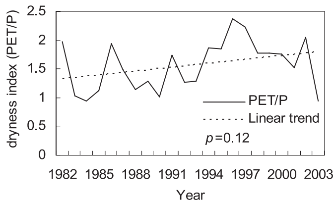
FIGURE 9. Annual Variation of Dryness Index (PET/P) With Linear Regression Line.
