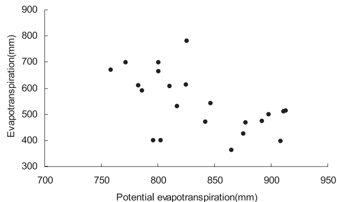
FIGURE 8. Scatter Plot of Actual Evapotranspiration Against Potential Evapotranspiration.
