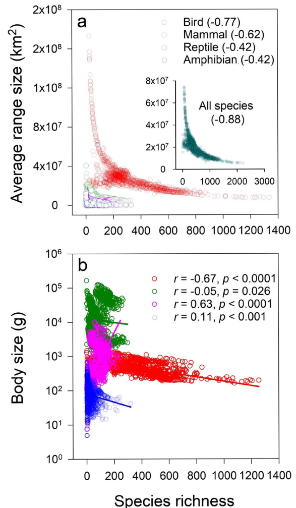
Fig. 3. a. The negative relationships ( r_s ) between species richness and average range size (km²) for each of the four terrestrial vertebrate groups (classes) and for all terrestrial vertebrates (inserted panel) around the world (in all cases, p < 0.001 ). b. The relationships between species richness and average body size for each of the four groups and all species of world terrestrial vertebrates.
