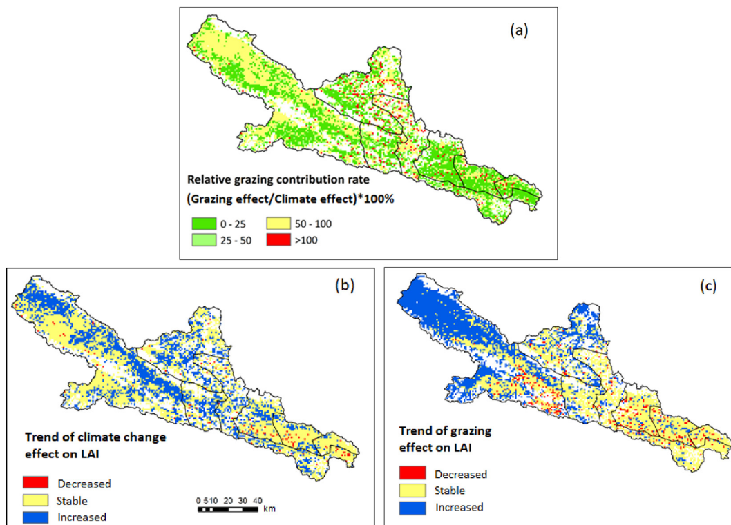
Fig. 8. Relative grazing contribution rate ( R_{GC} ) (a) and trends of effects of (b) climate change ( RC ) and (c) negative grazing ( RG ) over time on leaf area index (LAI) for the Upper Heihe River basin during 2001–2010. Three distinct areas in the trends of effect are identified as Decreased, Stable, and Increased. R_{GC} < 100 means that the grazing effect is less than the climate effect, otherwise the opposite.
