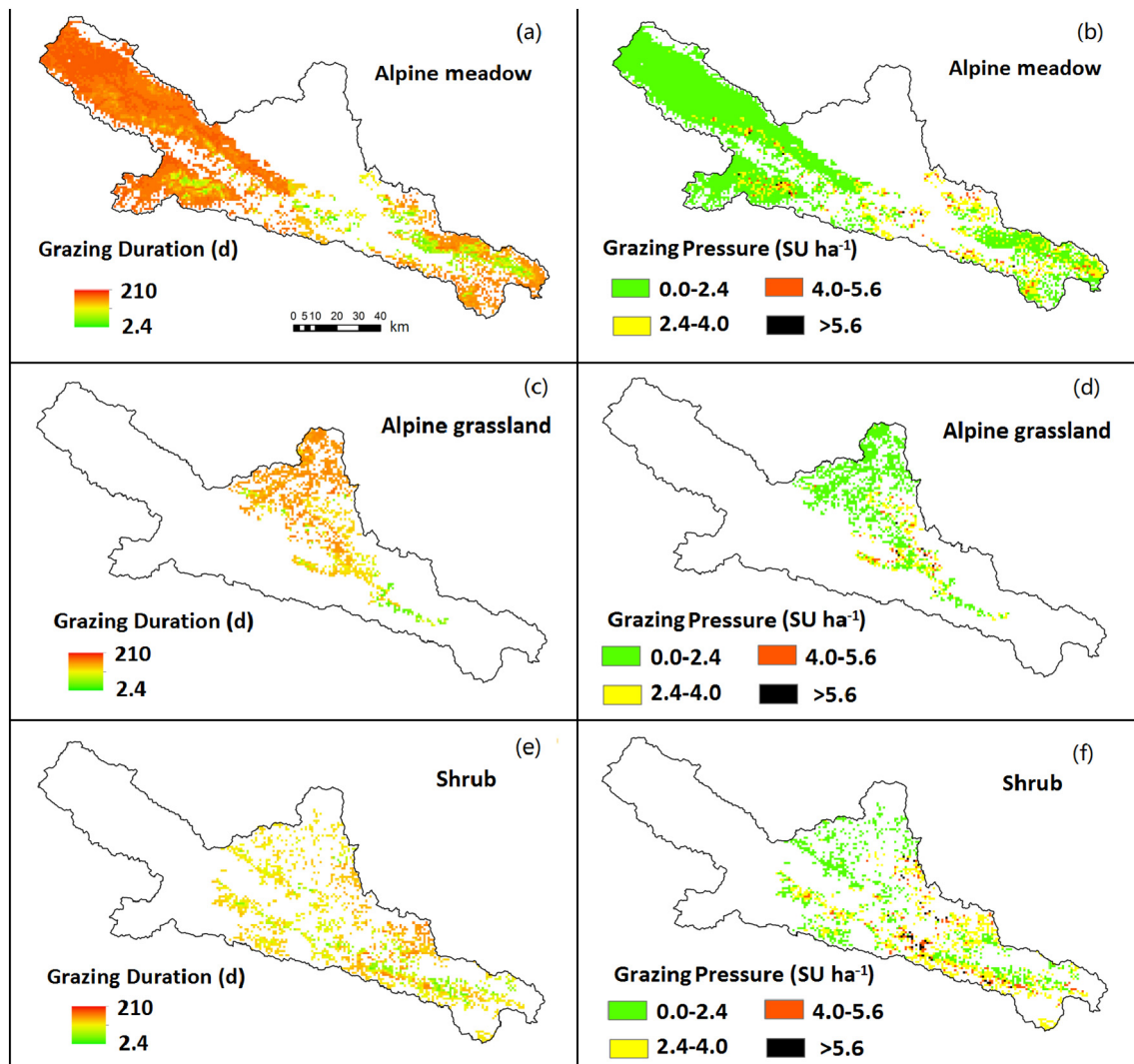
Fig. 6. Spatial patterns of annual mean grazing duration (GD, days), and grazing pressure (GP, SU\ ha^{-1} ) (2001–2010) with three grazing vegetation types of (a) and (b) alpine meadow, (c) and (d) alpine grassland, and (e) and (f) shrub, respectively.
