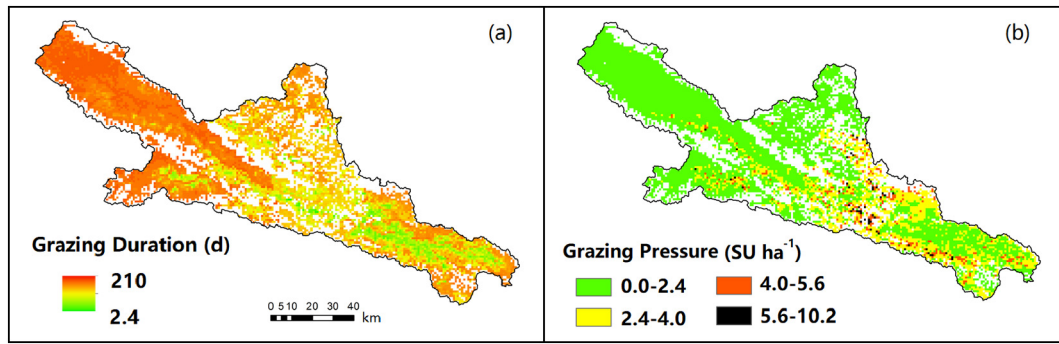
Fig. 5. Spatial patterns of annual (a) grazing duration (GD, days) and (b) grazing pressure (GP, SU\ ha^{-1} ) during 2001–2010.
