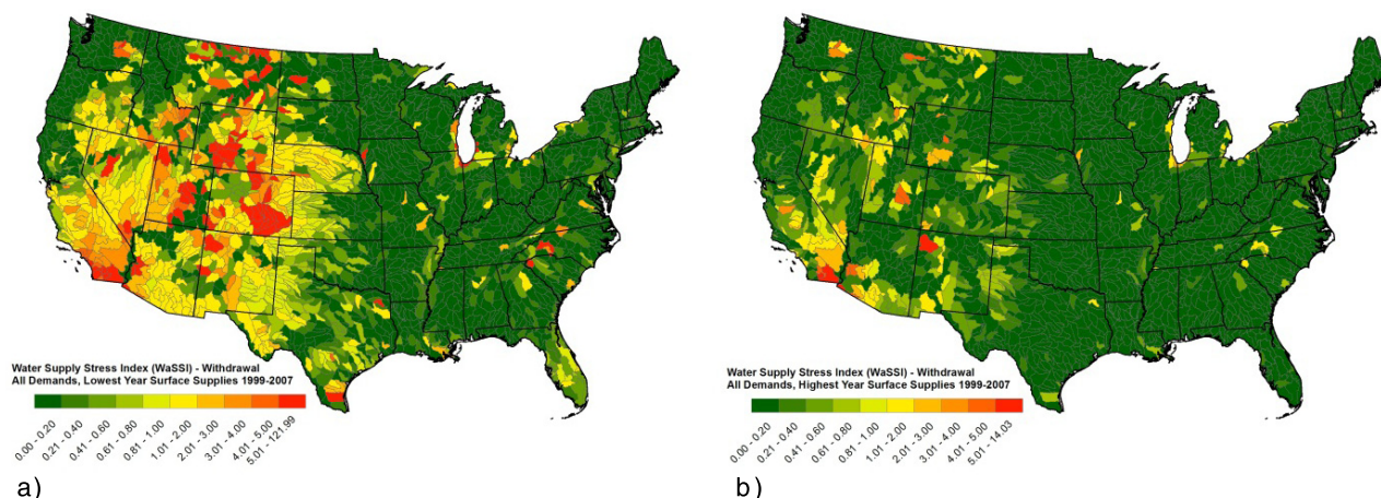
Figure 5. Withdrawal water supply stress index (WaSSI) sensitivity to low (L) and high (R) annual surface water supplies, 1999–2007. For each HUC-8 the lowest (a) and highest (b) annual flow occurring between 1999 and 2007 was selected and used to calculate WaSSI. This is not intended to represent large-scale spatial evolution of a low or high flow event, but to illustrate the sensitivity of WaSSI to surface supplies in different regions.
