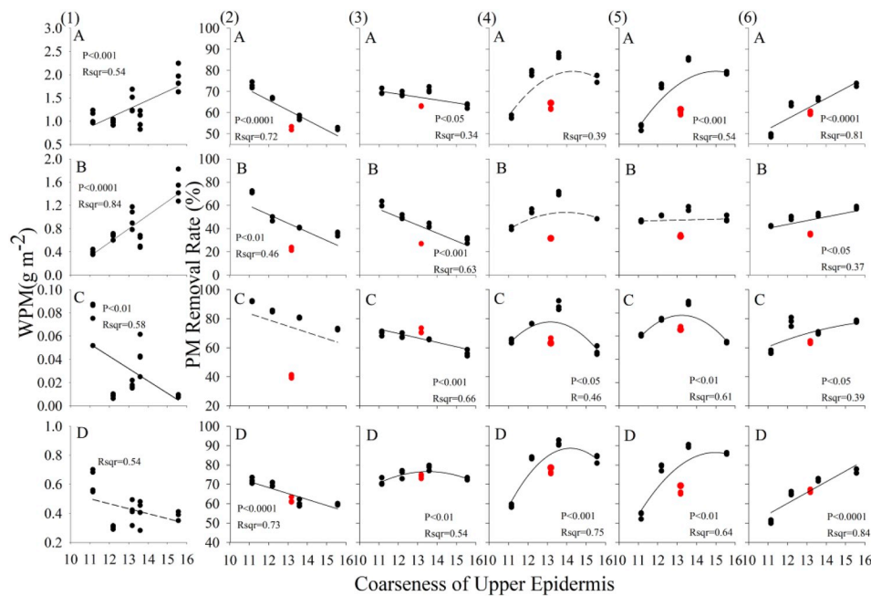
Fig. 6. Relationship between foliar PM and leaf coarseness. Panels (1) WPM, (2)–(6) representing PM removal rate for rainfall intensities of: (2) 10 mm h -1 , (3) 20 mm h -1 , (4) 40 mm h -1 , (5) 50 mm h -1 and (6) 72 mm h -1 . A to D in each panel represent different PM sizes: (A) TSP, (B) PM10-100, (C) PM2.5-10, and (D) PM2.5. Each leaf coarseness has three points representing replicate samples and the curve was fitted using only black plots (representing the other four plants besides Sophora japonica ).
