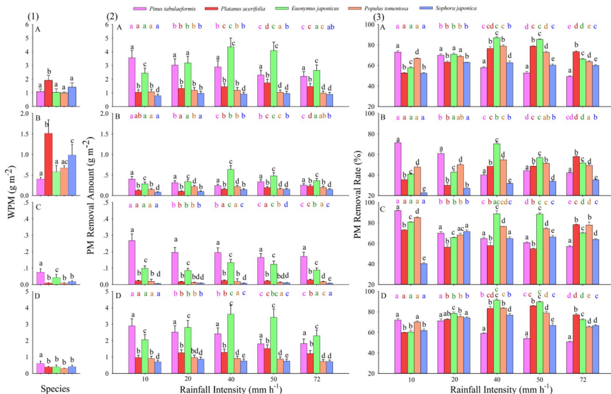
Fig. 2. Panel (1) represents WPM of different sizes. Panels (2) and (3) represent different size PM removal by the different rainfall patterns: (2) PM removal amount and (3) PM removal rate. A to D in each panel represent different PM sizes: (A) TSP, (B) PM10-100, (C) PM2.5-10, and (D) PM2.5. Data are presented as mean \pm SE. The black letters indicate significant differences between different species, and the colored letters corresponding to each species indicate significant differences between different rainfall patterns.
