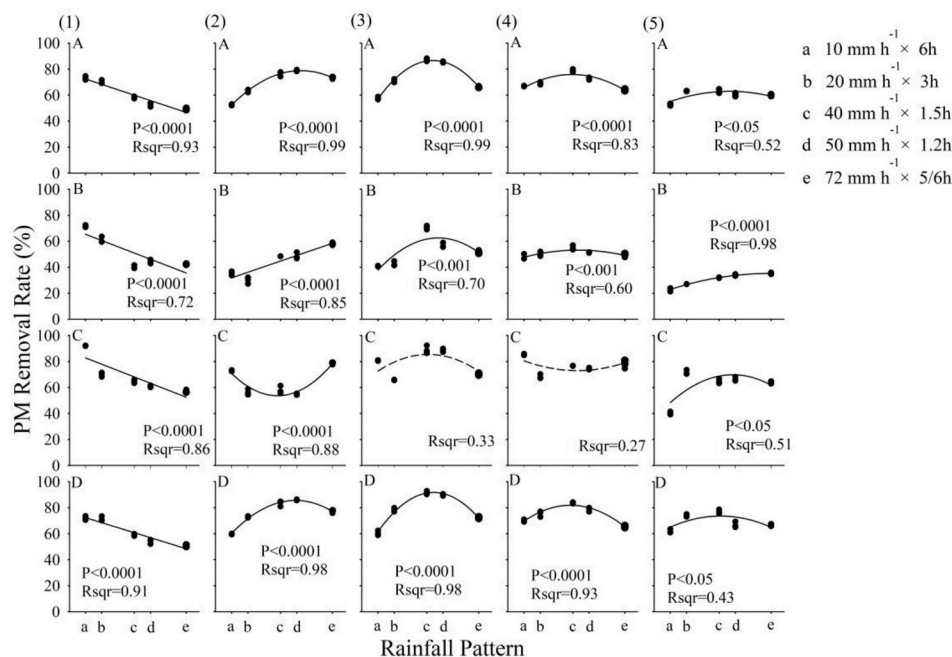
Fig. 4. Relationship between PM cumulative removal rate and rainfall duration for Pinus tabuliformis under different rainfall events. A to D represent different PM sizes: (A) TSP, (B) PM10-100, (C) PM2.5-10, and (D) PM2.5.
