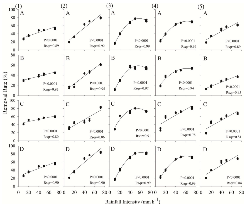
Fig. 3. Relationship between PM removal rate and rainfall intensity. Panels (1) to (5) represent different species: (1) Pinus tabuliformis , (2) Platanus acerifolia , (3) Euonymus japonicus , (4) Populus tomentosa , and (5) Sophora japonica . A to D in each panel represent different PM sizes: (A) TSP, (B) PM10-100, (C) PM2.5-10, and (D) PM2.5. Each intensity has three points representing the replicate samples.
