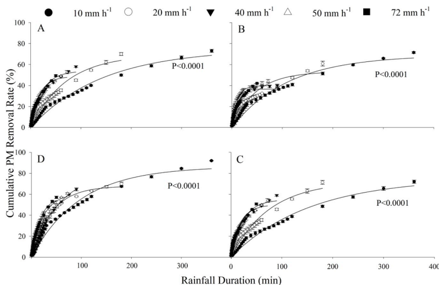
Fig. 4. Relationship between PM cumulative removal rate and rainfall duration for Pinus tabuliformis under different rainfall events. A to D represent different PM sizes: (A) TSP, (B) PM10-100, (C) PM2.5-10, and (D) PM2.5.
