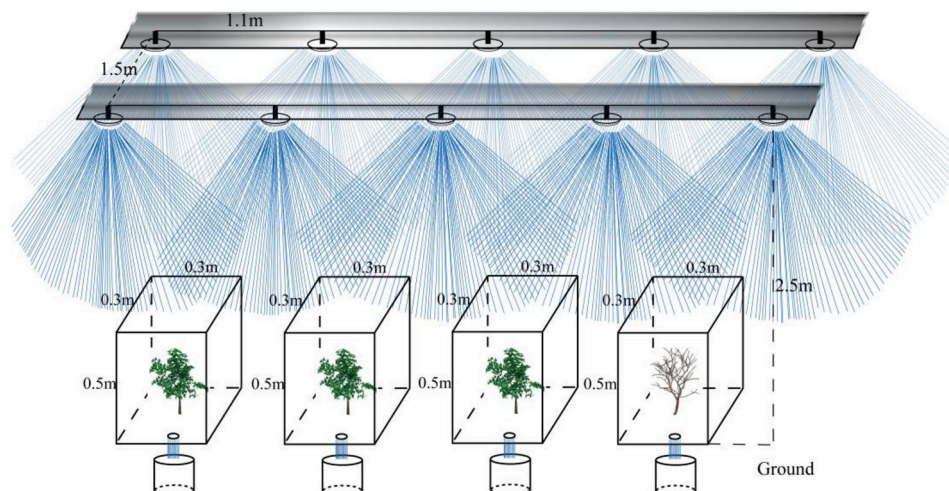
Fig. 1. The schematic diagram of rainfall experiment.
