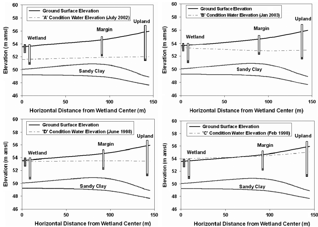
Figure 6. Cross-sectional view of a representative upland piezometer (4.6 m deep), margin piezometer (2.5 m), wetland piezometer (2.5 m), and the automatic digital recording pond gauge in the wetland (1.02 m) during the A–D cycle within the eastern transect (EF) in the depressional wetland. The role of the sandy clay sub-soil layer was to limit surface water–groundwater interaction even under relatively large hydraulic gradient conditions (e.g. condition C) and thus increasing the lateral groundwater flux
