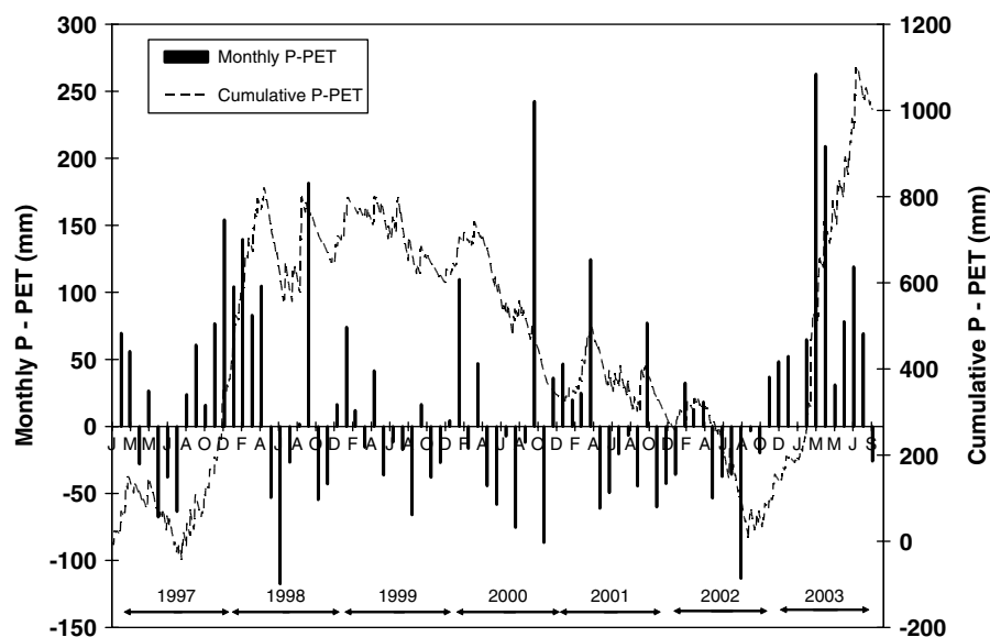
Figure 3. Monthly and cumulative differences between total precipitation (P) and potential evapotranspiration (ET) for 1997 to 2003 as obtained from an on-site rain gauge (and from the SC Department of Natural Resources SERCC weather station 24 km away in Bamberg, SC for 2000–2003), and calculated using the Hamon method (Federer and Lash, 1978; Sun et al. , 2002; Lu et al. , 2005), respectively
