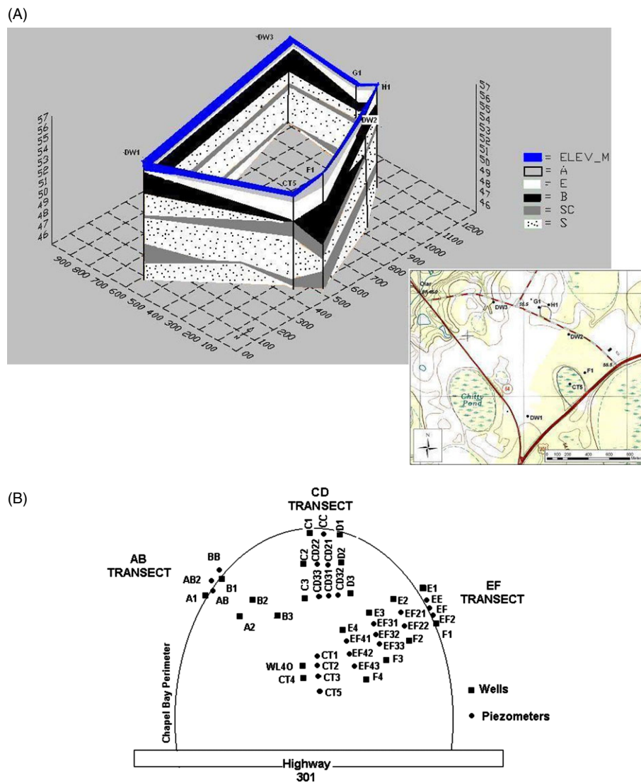
Figure 2. (A) Soil layers and shallow stratigraphy at study site, classified as follows: Horizon A (upland: sand; wetland: sandy loam to loamy sand), Horizon E (upland: sand; wetland: loamy sand), Horizon B (sandy clay loams), SC (sandy clay), S (sand). Labeled points represent well log locations. Elev_m refers to the elevation above mean sea level in metres. (B) Diagram showing piezometer and water-table well locations in and around the wetland
