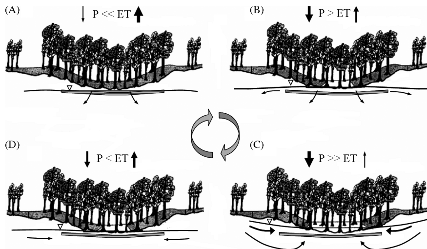
Figure 5. Conceptual hydrology responses to different P:ET conditions for a forested depressional wetland. Time scale varies from the annual (A: summer, B: autumn, C: winter, D: spring) to the weekly (high-intensity, convective rainstorm events in the summer cause P to exceed ET and induce the A–D cycle in the short-term). During drought conditions of 1999–2002 the cycle remained in the ‘A’ condition and cycled through to the ‘C’ condition within 2 weeks following a 160 mm rain event in March 2003 (Figure 4)
