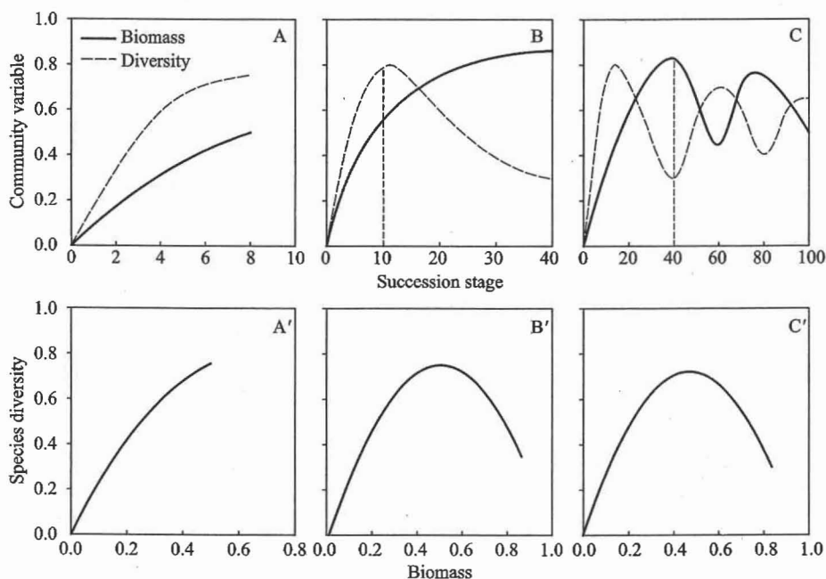
Fig. 3 - 1 Temporal dynamics of diversity and biomass and their relationships after a major disturbance. A, B, and C show the successional changes in diversity and biomass in the same ecosystem in 10, 40, and 100 years, respectively. A', B', and C' show the corresponding relationships between biomass and diversity in 10, 40, and 100 years, respectively. The difference between experimental and natural communities is that in experiments, aboveground biomass is removed for measuring productivity (but belowground biomass continues to accumulate; Guo et al. 2006) so the time needed for the hump-shaped curve to occur would be longer than natural settings where both above and belowground biomass is allowed to accumulate.
